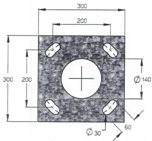
BASE PLATE DETAIL SCALE 1 : 8
